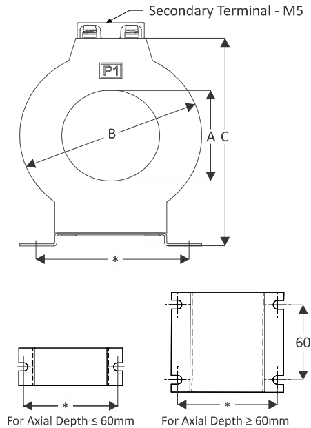
Mounting Dimensions
